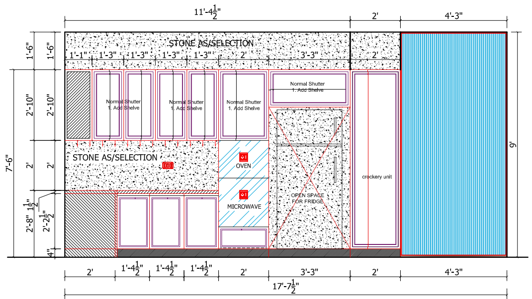
ELEVATION AT 'B'
